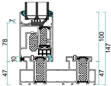
Aliplast Ultraglide HST
