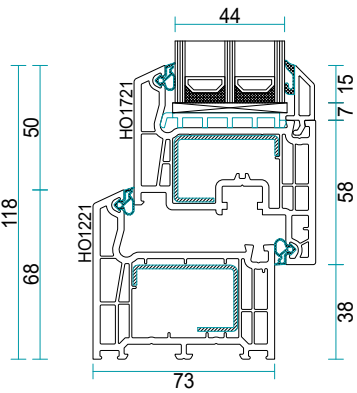
Salamander bluEvolution 73 P
