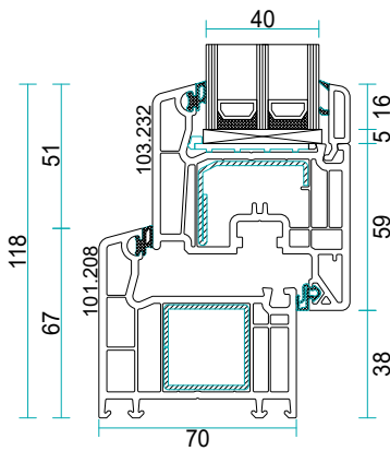
Veka Softline 70 P
