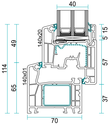
Aluplast Ideal 4000
