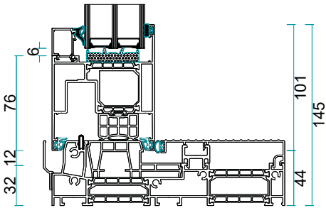
Aluplast Imperial 65
