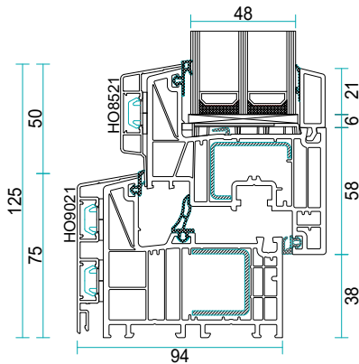
Salamander bluEvolution 82 MD Aluschale
