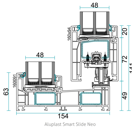
Aluplast Smart Slide Neo
