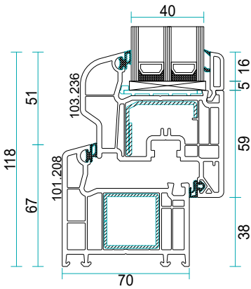
Veka Softline 70 O
