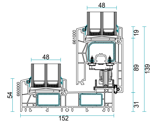
Salamander EvolutionDrive Plus+
