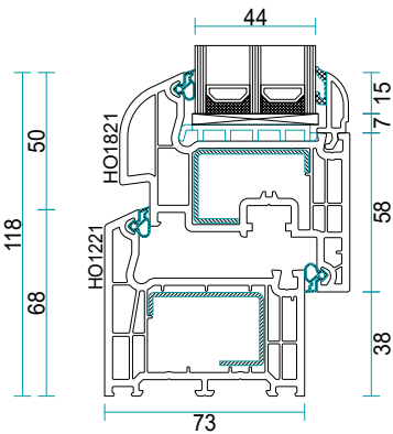
Salamander bluEvolution 73 O
